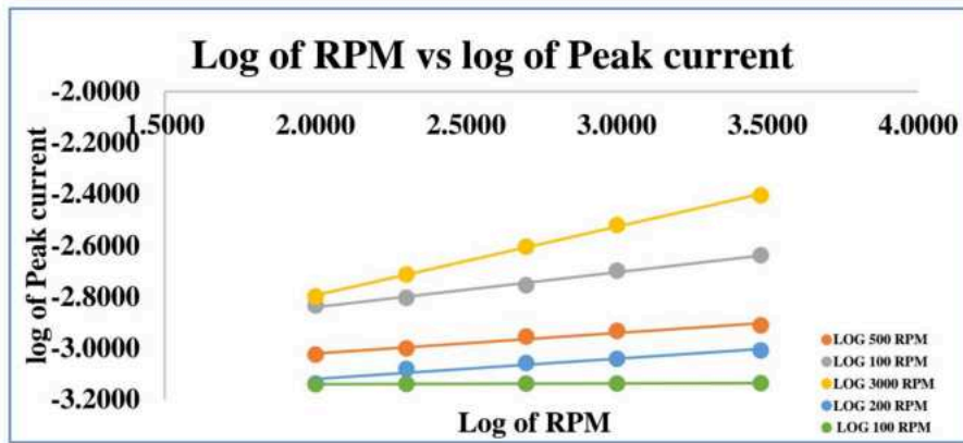
Figure 21 : log of RPM vs log of peak current for PPD 1.25 mM to 20.0 mM PPD coated PANI.
