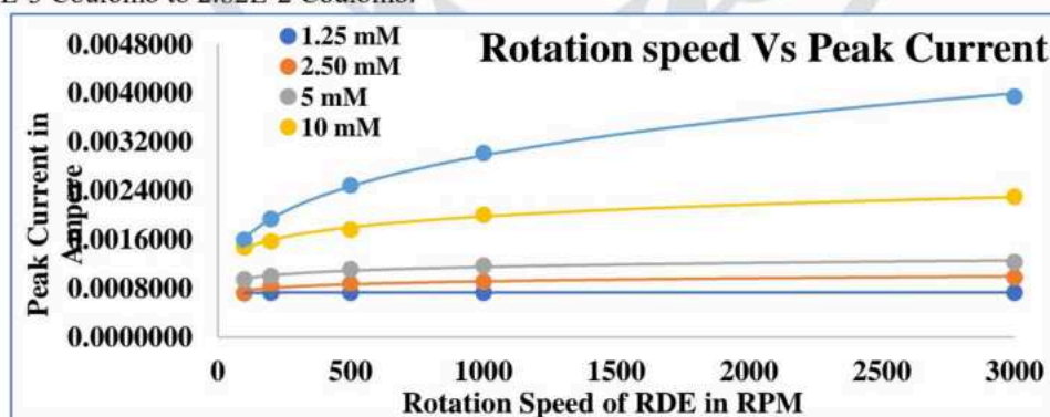
Figure 18: Plot of Rotation speed of RDE vs Peak current.
